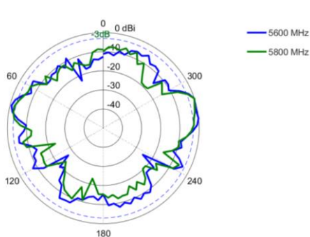
Elevation 1: 5600 – 5800 MHz
