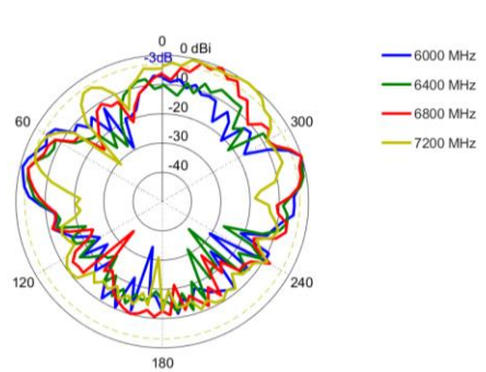
Elevation 1: 6000 – 7200 MHz
